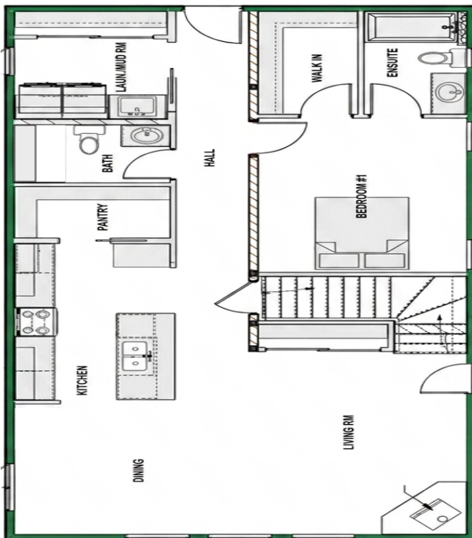
THE EVERWOOD | 46' X 25' | 1640 sq. ft. | 3 Bedroom s | 3 Bathroom s |
