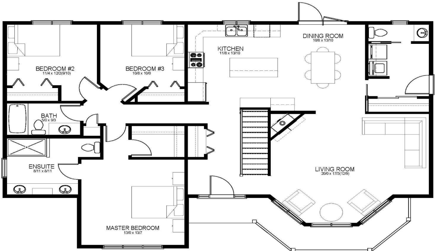
THE ROCKGLEN | 54' X 36' | 1675 sq.ft. | 3 Bedroom s | 3 Bathroom s |
